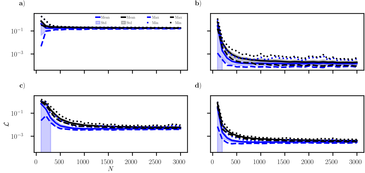
Figure 7: ExtremONet train loss (blue) and test loss (black) mean, standard deviation, maximum, and minimum with respect to the number of training points N (100 repeats). The y-scale is \log_{10} -scale NMSE. a) Lorenz-63 system. b) Gravity pendulum ODE with GRF ( t ). c) Parametrized Sine-Gordon PDE. d) Diffusion PDE with GRF ( x ).
