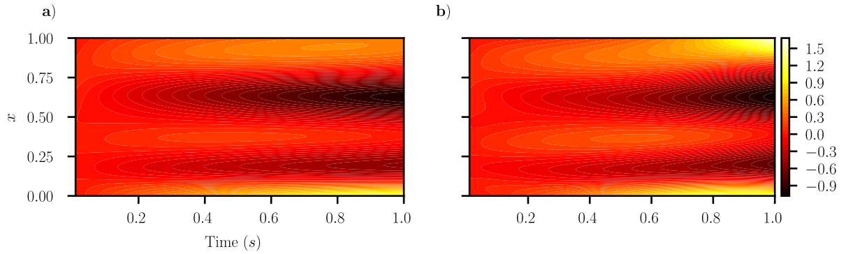
Figure 13: In-phase-space ExtremONet trajectory generation of a diffusion system with GRF length scale l = 0.1 and drift coefficient of d = 1 . a) Real time series. b) Predicted time series.
