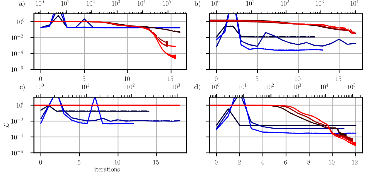
Figure 2: Train- and validation loss history (filled and dotted line) of three DeepONet (red) and three ExtremONets (blue). Model size is tied to colour shade. The upper x-axis represent DeepONet training iterations, lower x-axis represents Ridge Regression regularization parameter search iterations. The y-axis is log 10 -scale NMSE. a) Lorenz-63 system. b) Gravity pendulum ODE with GRF (t). c) Parametrized Sine-Gordon PDE. d) Diffusion PDE with GRF (x).
