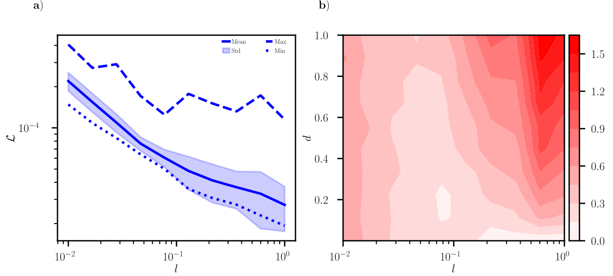
Figure 8: ExtremONet in phase space, trained on a diffusion system with spatial GRF; 100 repeats. a) Train loss mean, standard deviation, maximum and minimum with respect to the GRF length scale l \in [0.01, 1] , The y-scale is \log_{10} -scale NMSE. b) \log_{10}(\mathcal{L}_{test}/\mathcal{L}_{train}) with respect to the train- and test GRF length scale ( l \in [0.01, 1] ) on the x-axis, and the test drift amount ( d \in [0, 1] ) on the y-axis, The colorbar is \log_{10} -scale NMSE.
