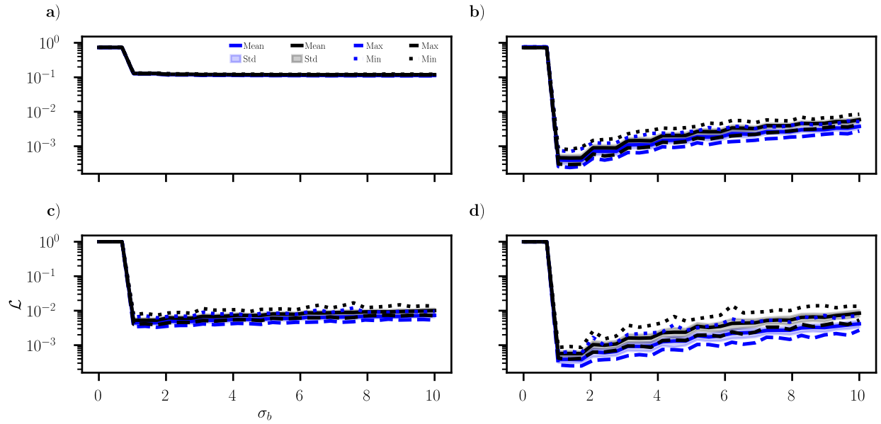
Figure 15: ExtremONet train loss (blue) and test loss (black) mean, standard deviation, maximum, and minimum for various branch scale \sigma_b (100 repeats). The y-scale is \log_{10} -scale NMSE. a) Lorenz-63 system. b) Gravity pendulum ODE with GRF (t). c) Parametrized Sine-Gordon PDE. d) Diffusion PDE with GRF (x).
