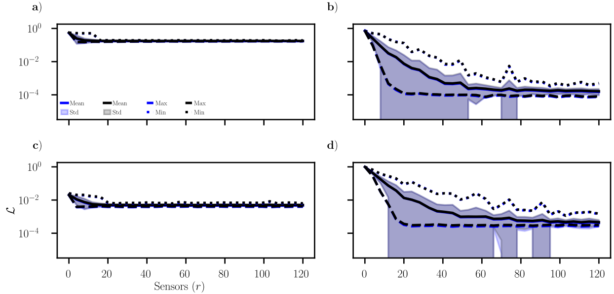
Figure 6: ExtremONet train loss (blue) and test loss (black) mean, standard deviation, maximum, and minimum with respect to the amount of sensors (100 repeats). The y-scale is \log_{10} -scale NMSE. a) Lorenz-63 system. b) Gravity pendulum ODE with GRF (t). c) Parametrized Sine-Gordon PDE. d) Diffusion PDE with GRF (x).
