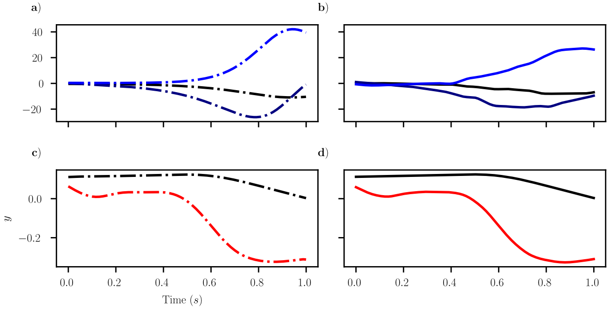
Figure 11: Hyperparameter-searched ExtremONet ODE predictions. a) Real Lorenz-63 system realization. b) Prediction of Lorenz-63 system realization; \sigma_t = 6.4 , \sigma_b = 6.1 , c_b = 1 , validation NMSE = 2.3 \cdot 10^{-2} . c) Real gravity pendulum ODE with GRF (t) realization. d) Prediction of gravity pendulum ODE with GRF (t) realization; s_t = 9.6 , s_b = 0.007 , c_b = 27 , validation NMSE = 8.7 \cdot 10^{-5} .
