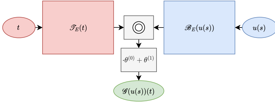
Figure 1: ExtremONet diagram.
