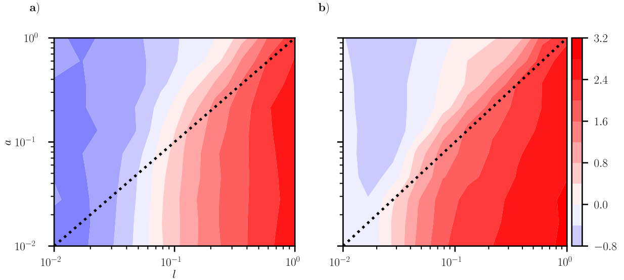
Figure 17: ExtremONet out-of-function-space dynamical drift performance, measured by \log_{10}(\mathcal{L}_{test}/\mathcal{L}_{train}) . Train GRF scale ( l \in [0.01, 1] ) on the x-axis, and test sinc parametrization ( a \in [0.01, 1] ) on the y-axis; 100 repeats. a) Gravity pendulum ODE with GRF (t). b) Diffusion PDE with GRF (x).
