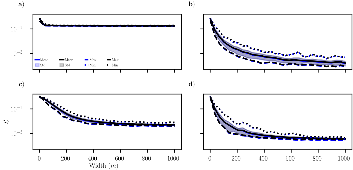
Figure 4: ExtremONet train loss (blue) and test loss (black) mean, standard deviation, maximum, and minimum with respect to width (100 repeats). The y-scale is \log_{10} -scale NMSE. a) Lorenz-63 system. b) Gravity pendulum ODE with GRF (t). c) Parametrized Sine-Gordon PDE. d) Diffusion PDE with GRF (x).
