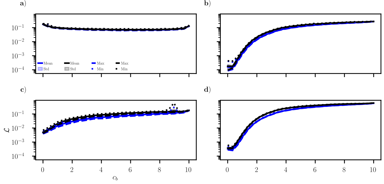
Figure 16: ExtremONet train loss (blue) and test loss (black) mean, standard deviation, maximum, and minimum for various branch connectivity c_b (100 repeats). The y-scale is log 10 -scale NMSE. a) Lorenz-63 system. b) Gravity pendulum ODE with GRF (t). c) Parametrized Sine-Gordon PDE. d) Diffusion PDE with GRF (x).
