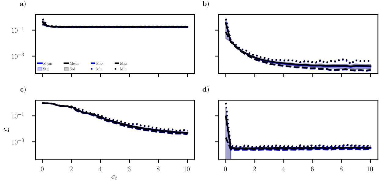
Figure 14: ExtremONet train loss (blue) and test loss (black) mean, standard deviation, maximum, and minimum for various trunk scale \sigma_t (100 repeats). The y-scale is \log_{10} -scale NMSE. a) Lorenz-63 system. b) Gravity pendulum ODE with GRF (t). c) Parametrized Sine-Gordon PDE. d) Diffusion PDE with GRF (x).
