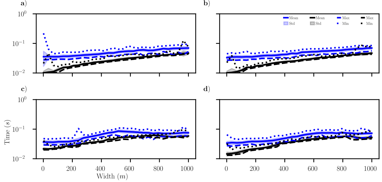
Figure 5: ExtremONet mean and standard deviation train- and prediction time with respect to width (100 repeats). The y-scale is \log_{10} -scale seconds. a) Lorenz-63 system. b) Gravity pendulum ODE with GRF (t). c) Parametrized Sine-Gordon PDE. d) Diffusion PDE with GRF (x).
